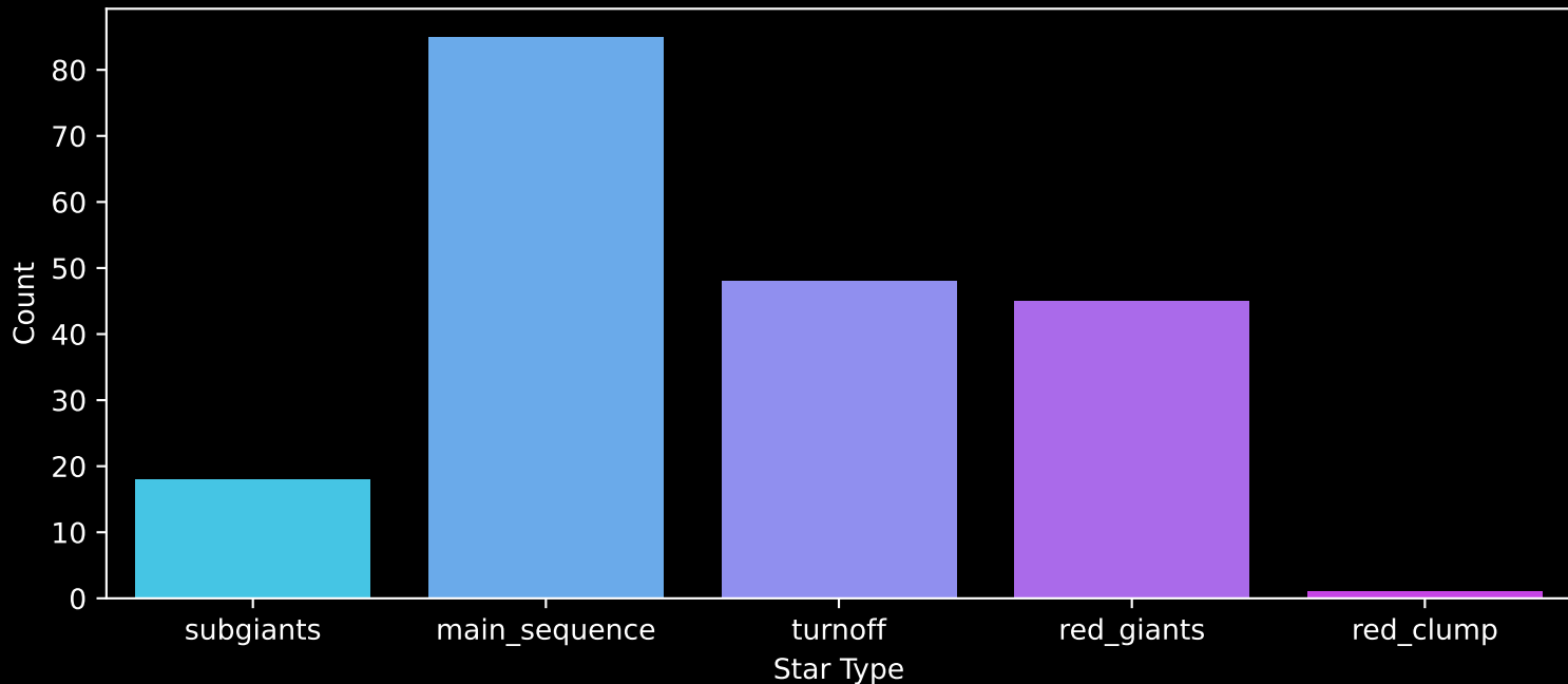
APOGEE DR17 Field: [182-45_MGA] Count plot of Star Type
