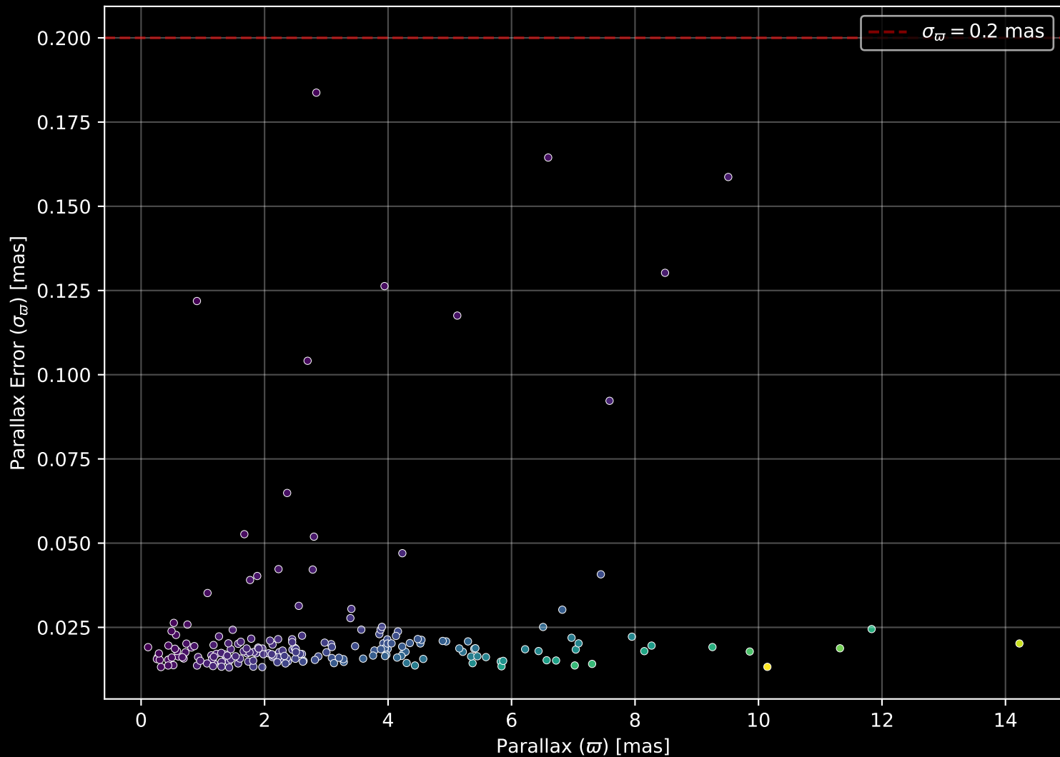
APOGEE DR17 Field: [182-45_MGA] Parallax Quality (n= 197)
