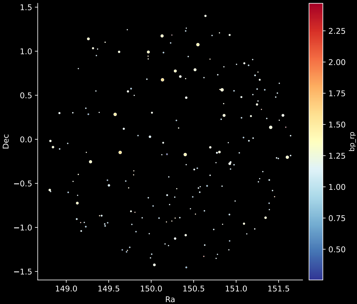
APOGEE DR17 Field: [182-45_MGA] Stars: 197
