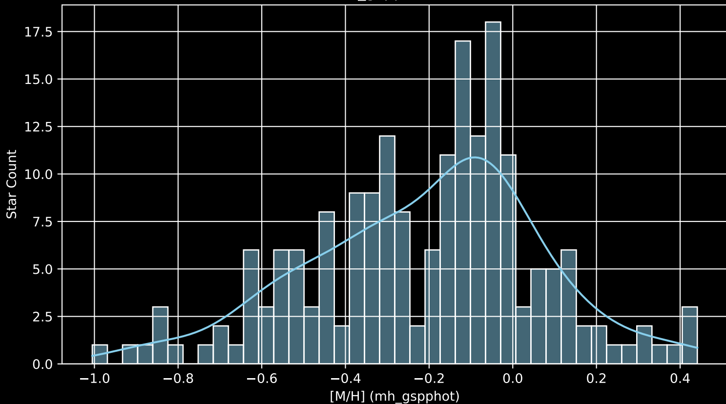
APOGEE DR17 Field: [182-45_MGA [M/H] (mh_gspphot) (n= 192)
