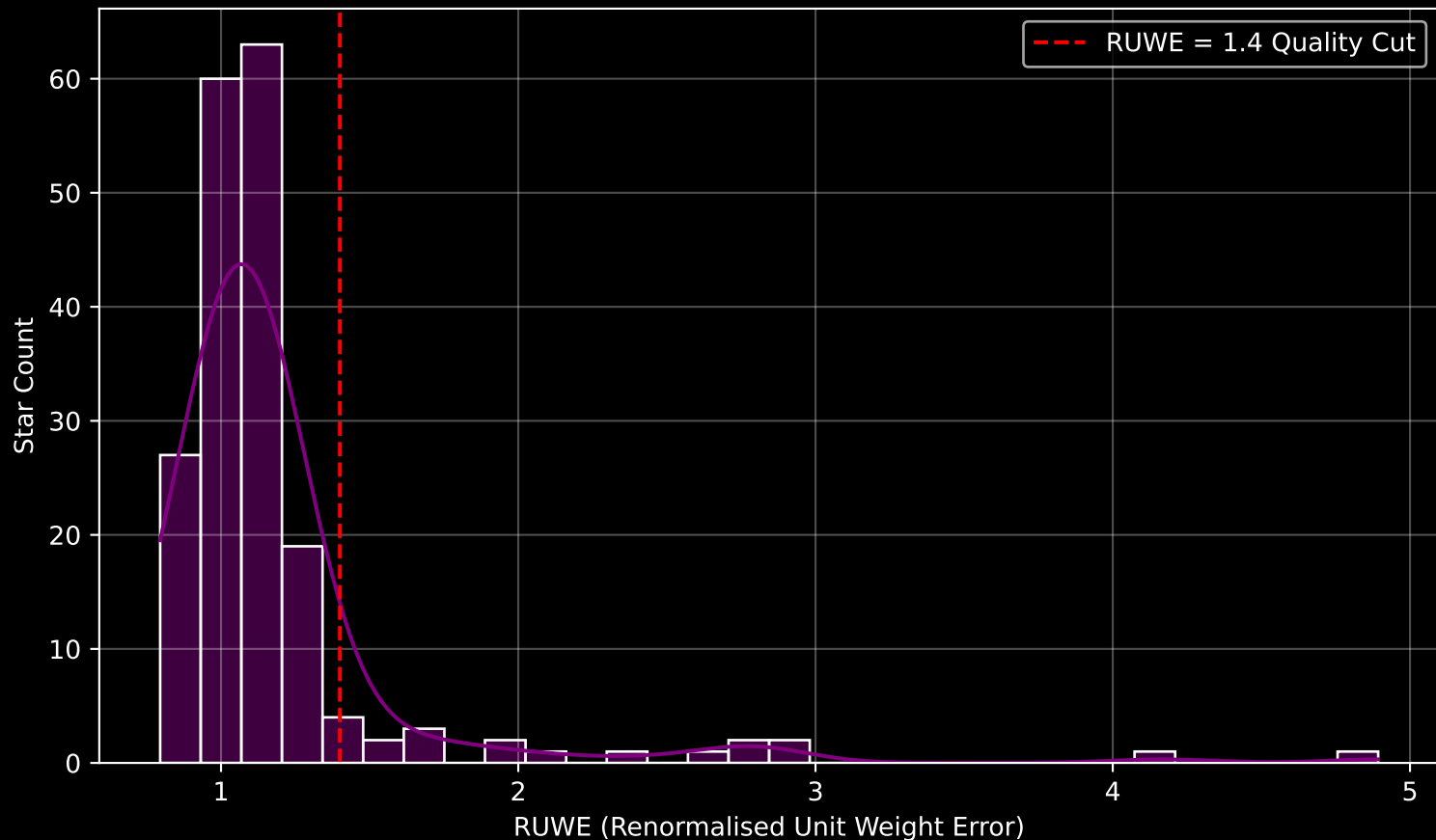
GAPOGEE DR17 Field [182-45_MGA] RUWE Distribution (n= 189)
