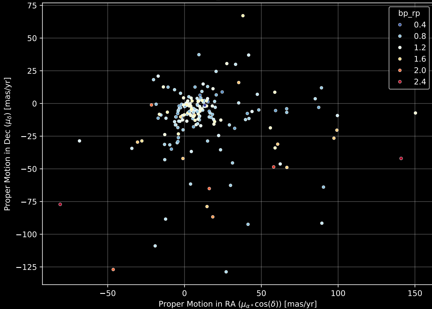
APOGEE DR17 Field: [182-45_MGA] Proper Motion Diagram (n= 197)
